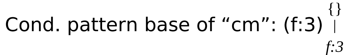
cm -conditional FP-tree
